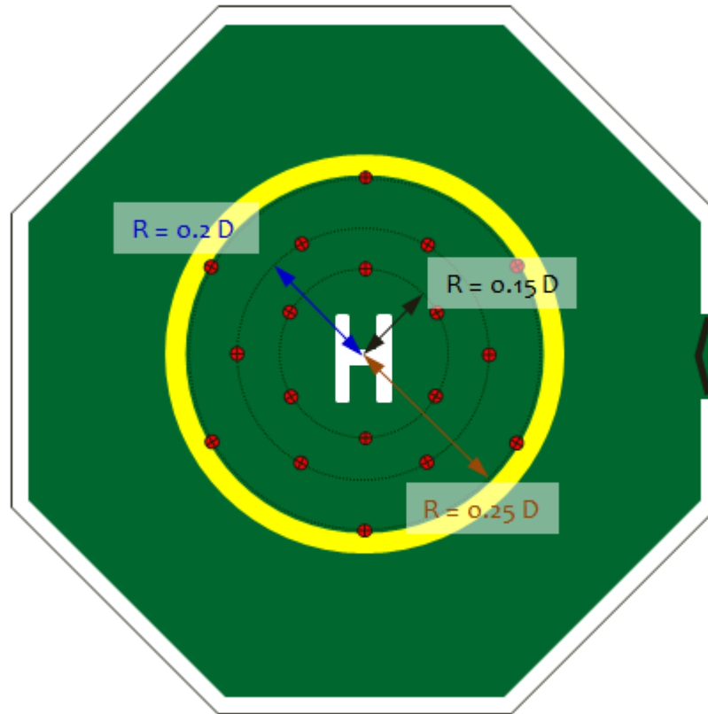
Figure 15 — Tie-down Locations
