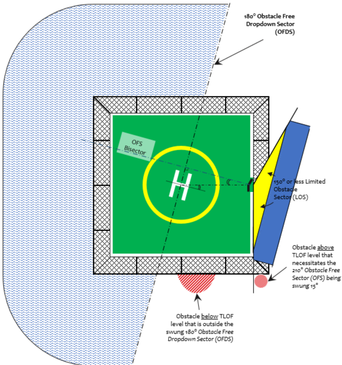
Figure 3.4.5 OFS Sector Swung by 15 Degrees
