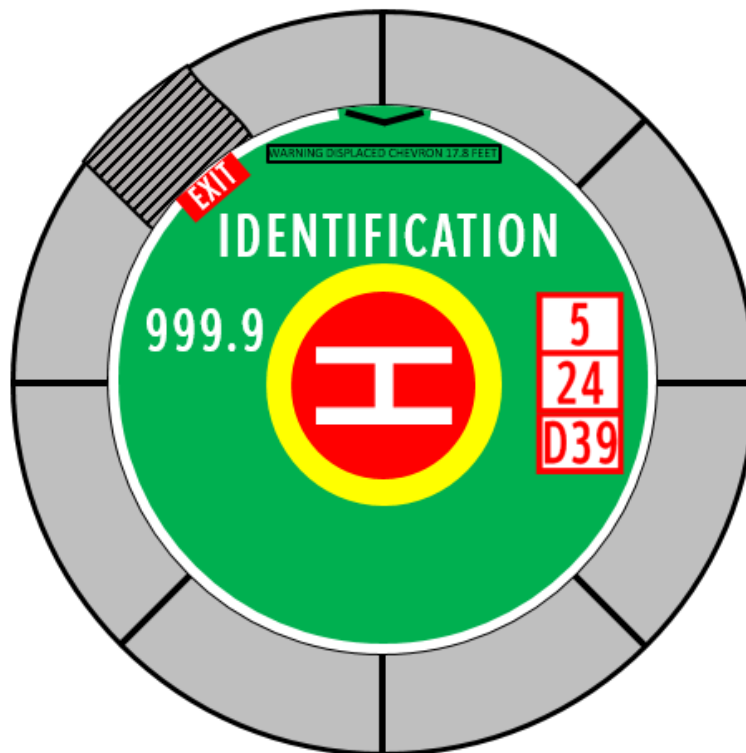
Figure 4.5D D-value, TLOF Size and Weight Markings for a 0.62D TLOF with a Circular TLOF
